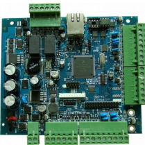
RLIFT-CF/IP(2.0A)-PCB
